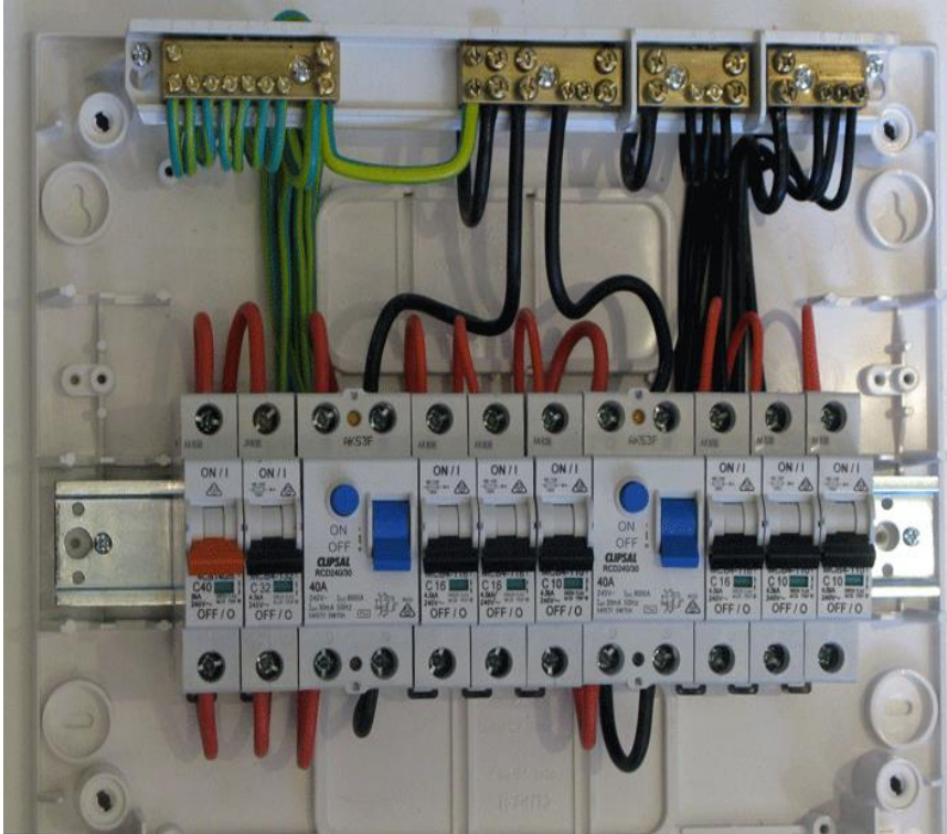
MCB PANEL
